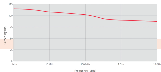
7400 series - Ultra soft shield
