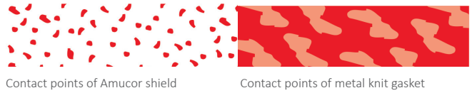
Contact points of Amucor shield
