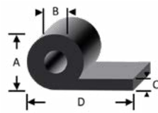
P profile (P)
