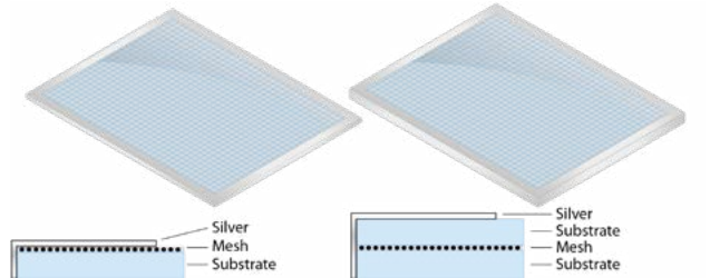
SB : Silver busbar (Single layer) Wire mesh fixed onto one side of glass or plastic substrate. SB : Silver busbar (Double layer) Wire mesh fixed between two layers of glass or plastic substrate.
