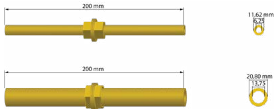
Waveguide brass 7855-32,90 & 7855-47,60
