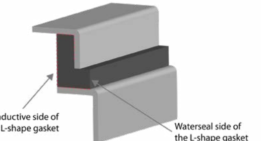
Figure 54: Example image of a L-shape gasket
