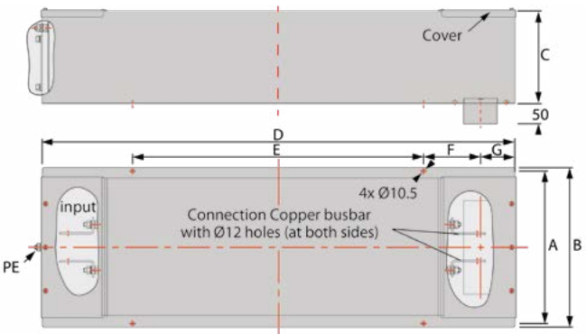
Outline drawing 2
