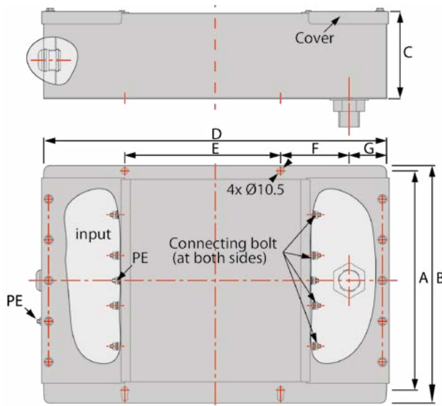
Outline drawing 3
