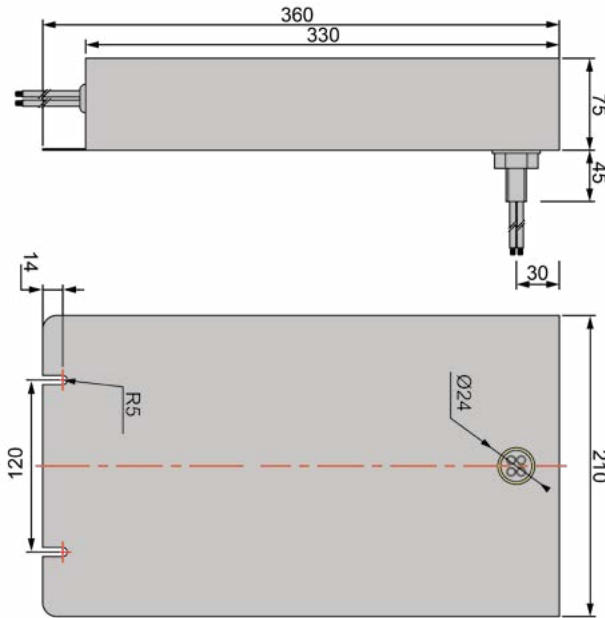
Outline drawing 6
