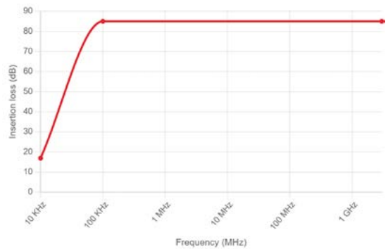
8070-2-16 pluggable TEMPEST filter
