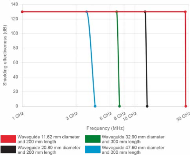
Waveguide brass 7855-32,90 & 7855-47,60
