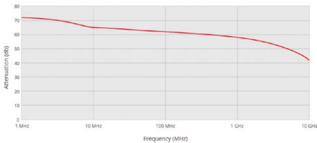
4730 - 4760 series - Wrapshield (E field)
