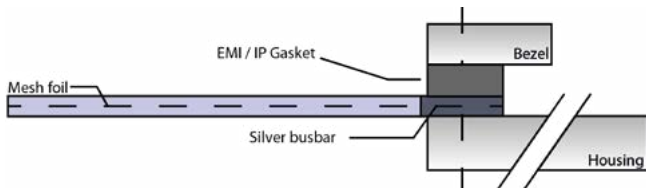
Mounting example 3 Standard Mesh foil mounted in a clamping construction with an EMI gasket. A water seal is possible here.
