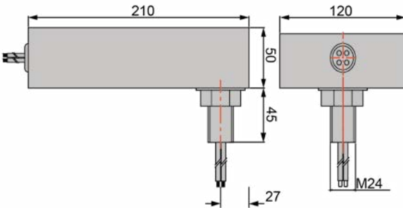
Outline drawing 4
