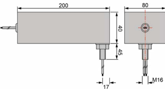
Outline drawing 3
