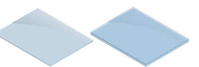
NO : No contact edge (Single layer) Wire mesh fixed onto one side of glass or plastic substrate. NO : No contact edge (Double layer) Wire mesh fixed between two layers of glass or plastic substrate.
