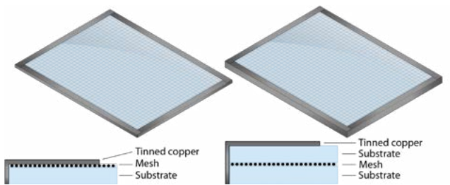
TC : Tinned copper busbar (Single layer) Wire mesh fixed onto one side of a glass or plastic substrate. With tinned copper edges for easy soldering and grounding. TC : Tinned copper busbar (Double layer) Wire mesh fixed between two glass or plastic substrate. With tinned copper edges for easy soldering and grounding.
