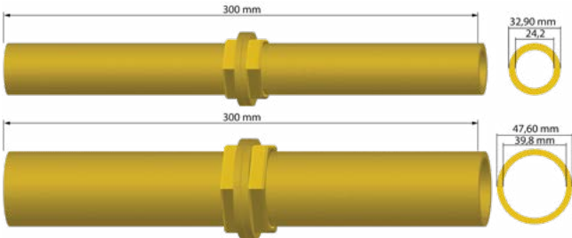
Waveguide brass 7855-32,90 & 7855-47,60
