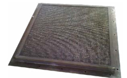
Figure 82: Picture of a EMP proof Honeycomb ventilation panel
