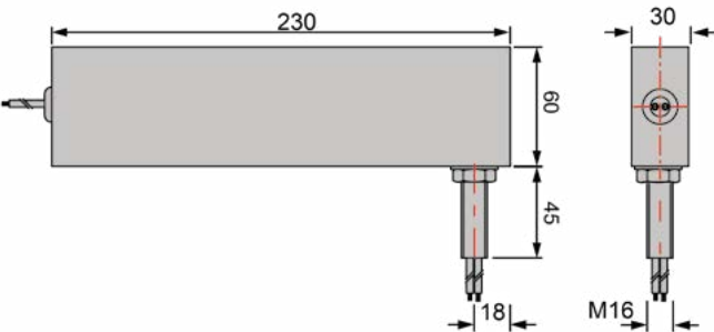
Outline drawing 1
