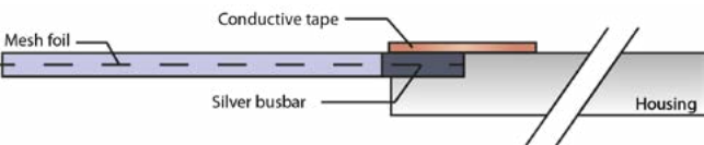
Mounting example 2 Mesh foil mounted with Conductive tape 3201
