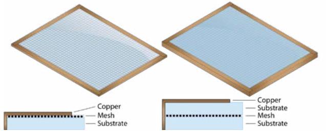
CO : Copper busbar (Single layer) Wire mesh fixed onto one side of glass or plastic substrate. CO : Copper busbar (Double layer) Wire mesh fixed between two layers of glass or plastic substrate.
