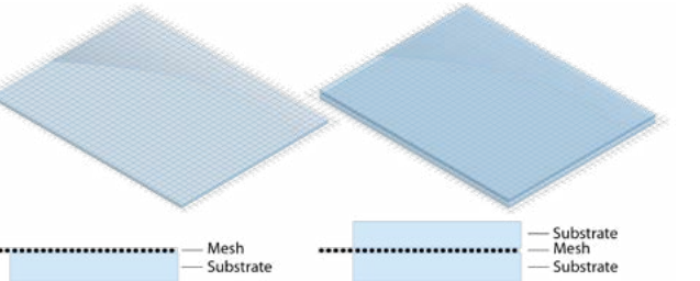
FM : Flying mesh (Single layer) Wire mesh fixed onto one side of glass or plastic substrate. FM : Flying mesh (Double layer) Wire mesh fixed between two layers of glass or plastic substrate.
