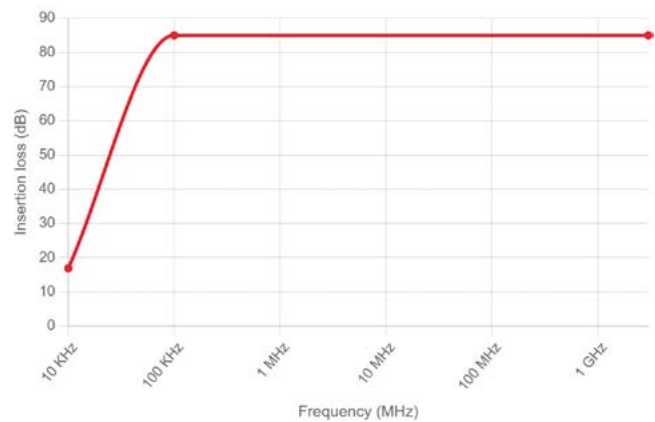
8070-2-16 pluggable TEMPEST filter
