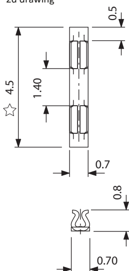
2d drawing
