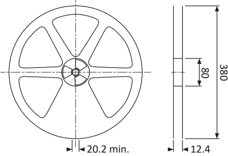
Plastic reel drawing
