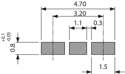
Recommended solder land size
