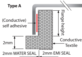
Type A: 2 mm waterseal and 2 mm conductive layer on the bottom; flange height can be specified
