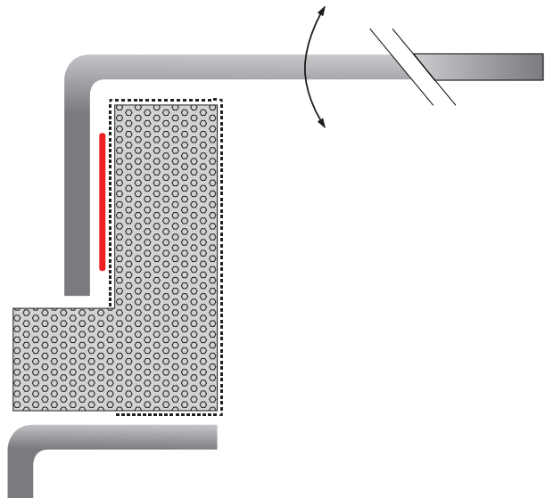
Technical drawing L-shape
