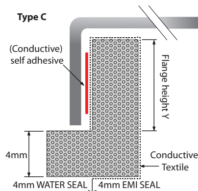
Type C: 4 mm waterseal and 4 mm conductive layer on the bottom; flange height can be specified
