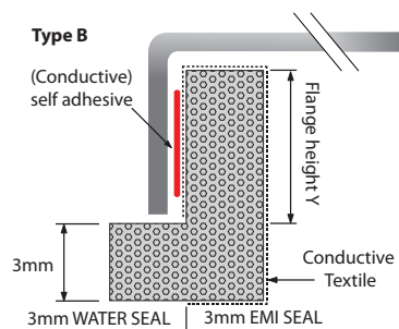
Type B: 3 mm waterseal and 3 mm conductive layer on the bottom; flange height can be specified
